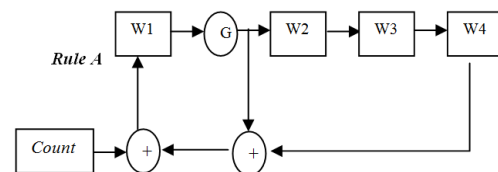
Gambar 4. Rule A
