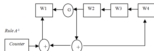
Gambar 6. Rule A -1
