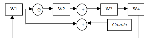
Rule B
